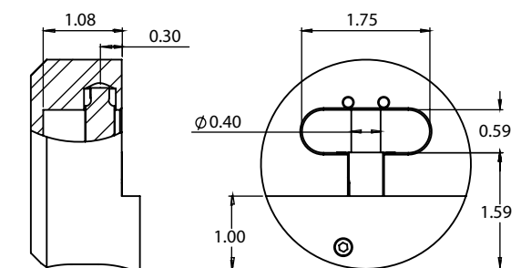
3/8" Diam. Shackle
